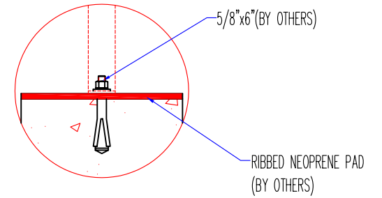
DETAIL A 1:10
