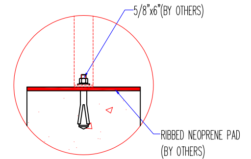
DETAIL A 1:10
